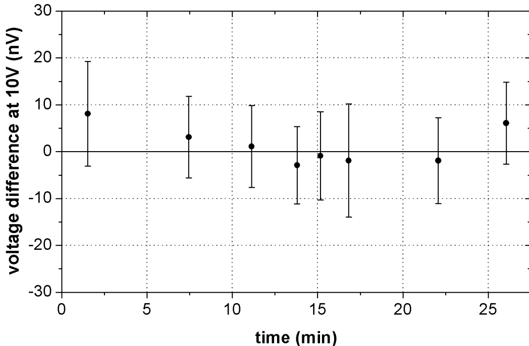
Fig. 4. Measurements of the direct comparison between a cryocooler-based and a liquid-helium-based Josephson voltage standard system at a voltage level of 10 V. The difference of the voltages was U_{\text{PTCS}} - U_{\text{LHeS}} = 1.3 nV with a combined standard measurement uncertainty of 2 nV.
